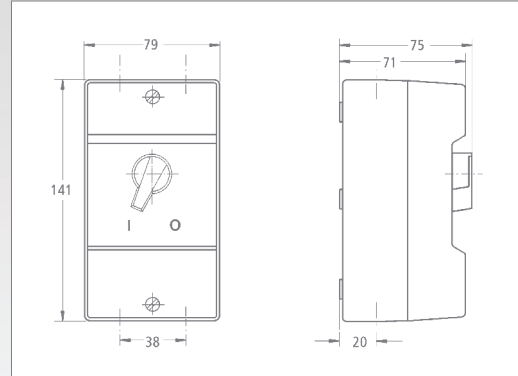
Enclosure H
