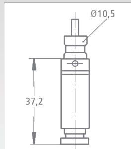
AEV 35
