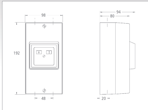
Enclosure B
