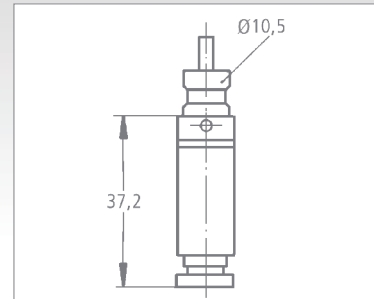
AEV 25
